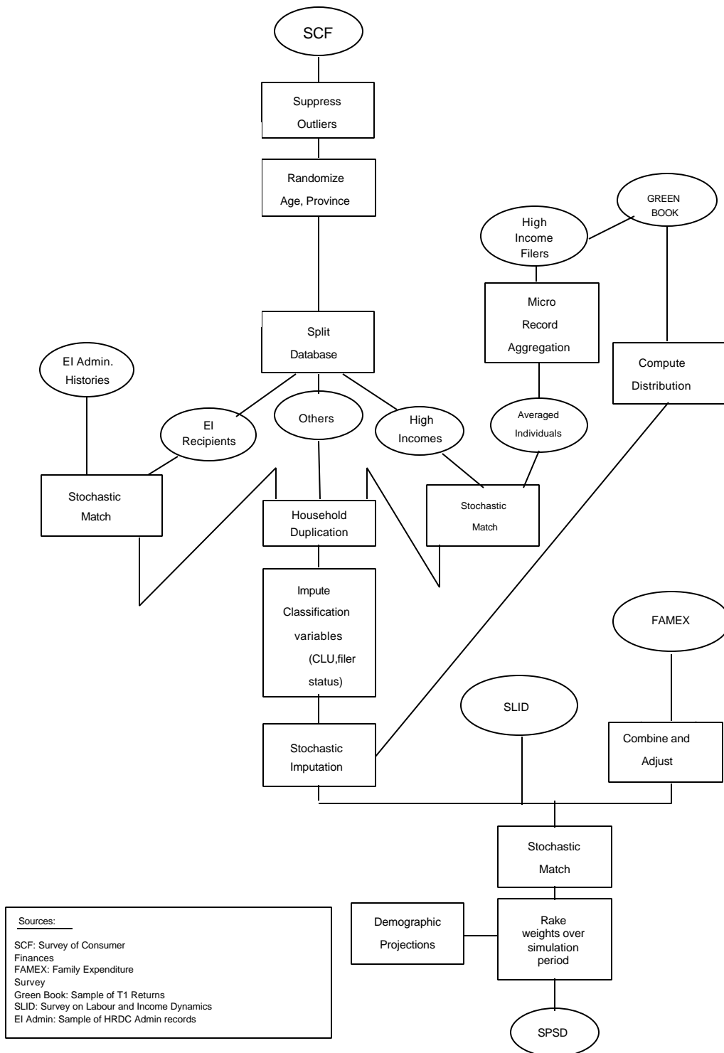
Figure 1: SPSP Database Creation Process The Host Data
